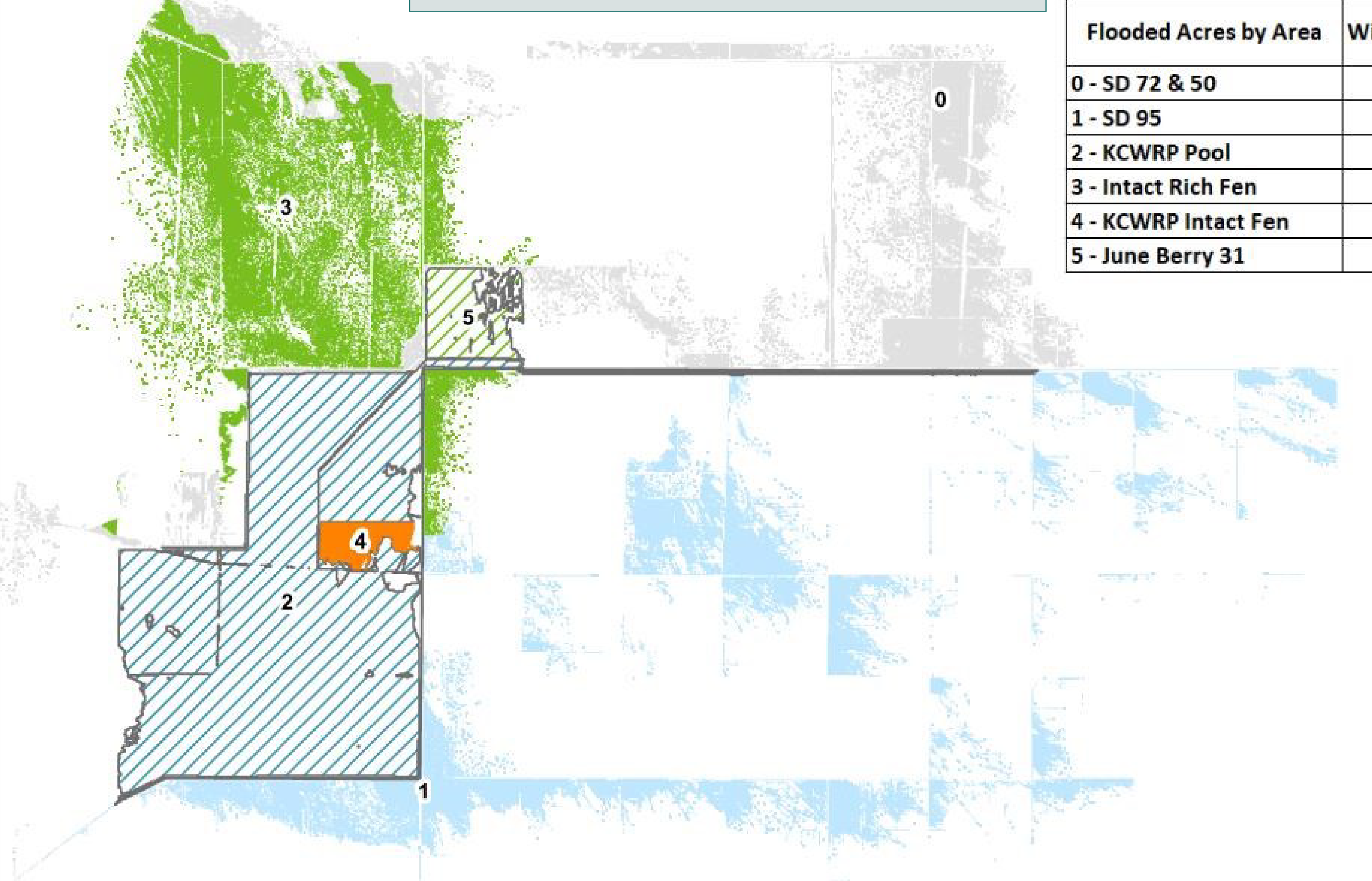
Proposed Conditions, 25-Year Event
